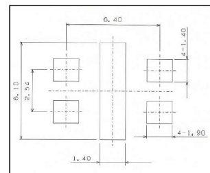
PIN CONNECTIONS
